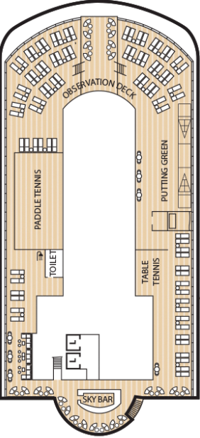
Deck 14
